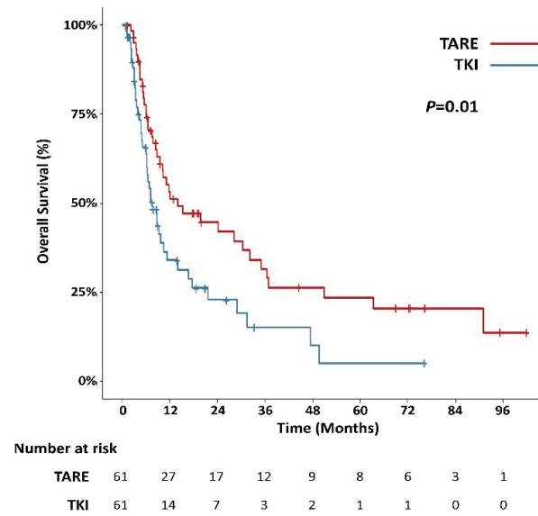
Supplementary Figure 3. Comparison of OS after excluding patients who received subsequent resection or RFA. After excluding 10 patients who underwent resection (n=8) or RFA (n=2) after TARE, OS was compared in an unmatched cohort (A) and balanced cohorts using IPTW (B) or PSM (C). No patients received subsequent resection or RFA in the TKI group. IPTW, inverse probability of treatment weighting; OS, overall survival; PSM, propensity score matching; RFA, radiofrequency ablation; TARE, transarterial radioembolization; TKI, tyrosine kinase inhibitor.
