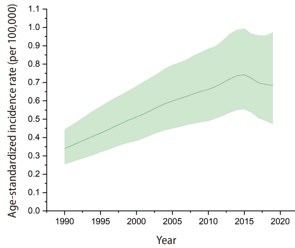
Supplementary Figure 6. Age-standardized incidence rate of liver cancer due to HBV in Australasia from 1990 to 2019. HBV, hepatitis B virus.
