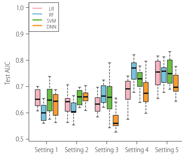
Supplementary Figure 5. Comparison of performance between machine learning models for settings 1–5 by iterating the process of splitting the total dataset into model development and test sets. AUC, area under the receiver operating characteristic curve; LR, logistic regression; RF, random forest; SVM, support vector machine; DNN, deep neural network.
